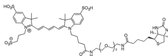
Chemical Structure:
