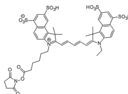
Chemical Structure:
