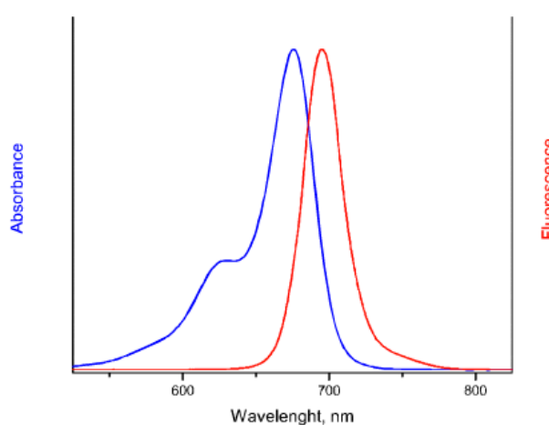
Absorption and Emission Spectra
