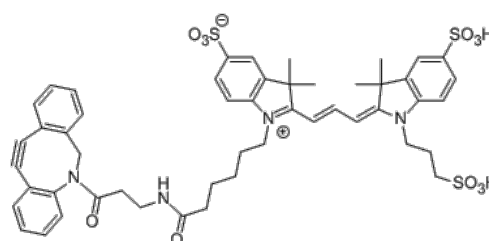
Chemical Structure:
