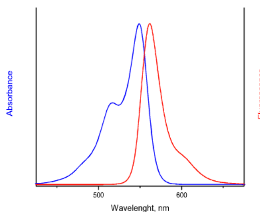
Absorption and Emission Spectra
